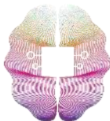
Artificial Intelligence
